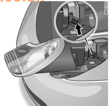
Litronic headlights
